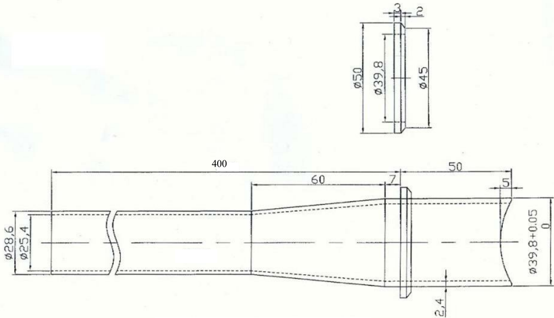
DRAWING TBE-STR-28.6-1.5-39.8-2.4-450
